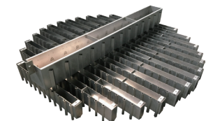
• Liquid Distributor
